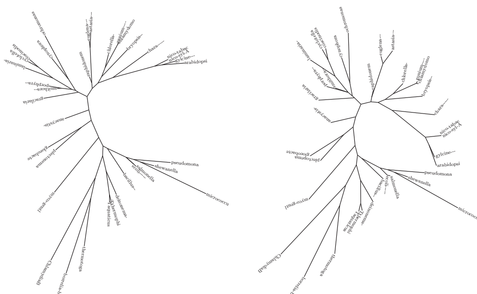
Figure 5.15 Radial tree layout with the same root as in Fig. 5.10 and leaf reordering for drawing those closely related near. The right drawing is with spreading.
