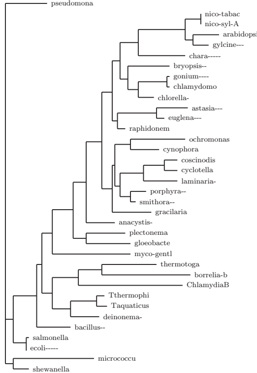
Figure 5.10 An example of a phylogenetic tree (phylogram, redrawn from [DS04]).
